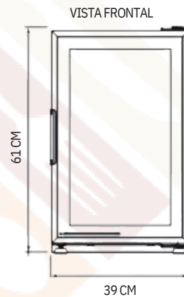
VISTA FRONTAL
